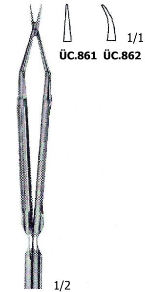
BROCK – 15 cm ÜC.861-ÜC.862
